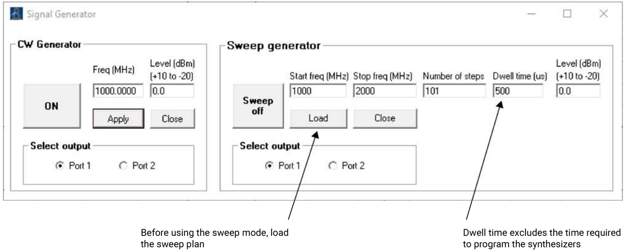
Signal generator utility control window
