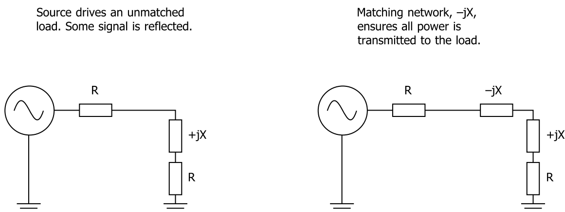
Matching a load for maximum power transfer
