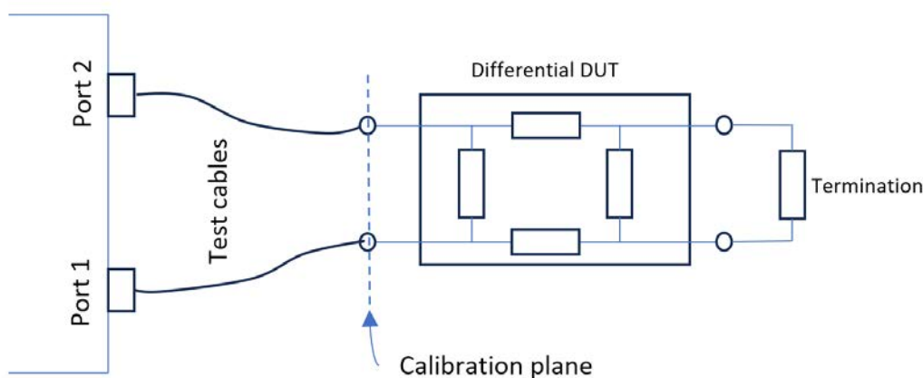
Differential reflection measurement connections
