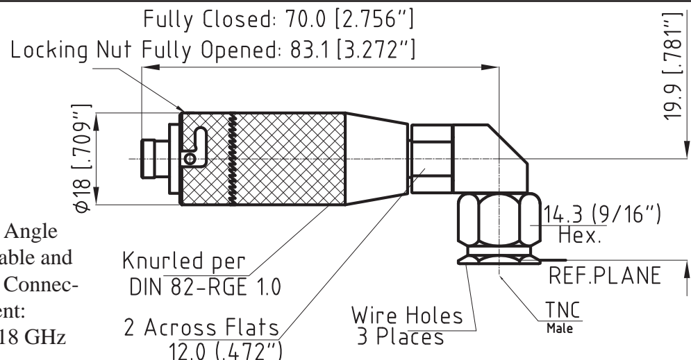
TNCm Right Angle Phase Adjustable and Self Locking Connector, Adjustment: 240° min. @18 GHz
