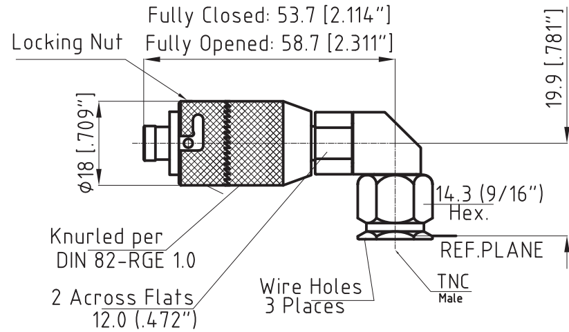
TNCm Right Angle Phase Adjustable and Self Locking Connector, Adjustment: 100° min. @18 GHz
