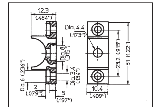
Bracket, Part No.: MB-0200-07 Material: Aluminum iridited
