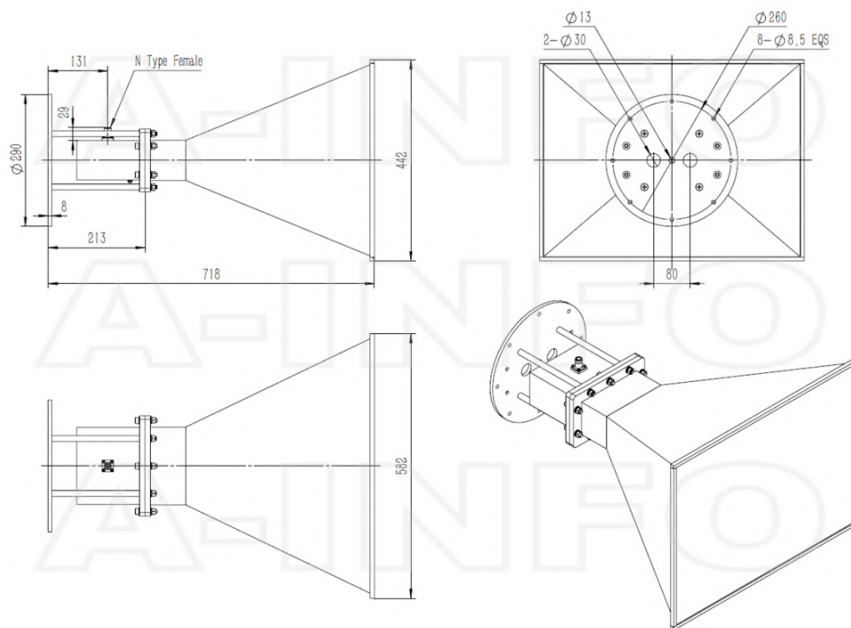
N-Female Output with Round Mounting Bracket & Radome (Option, P/N: LB-650-10-C-MB & LB-OH-650-15-C-NFSPO, Outdoor Application)
