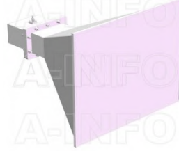
LB-OH-650-15-C-SFSPO Octave Horn Antenna 1-2GHz 15dB Gain SMA Female
