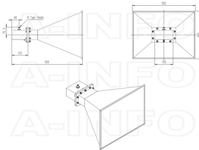
N-Female Output with Radome (Option, P/N: LB-OH-650-15-C-NFSPO, Outdoor Application)
