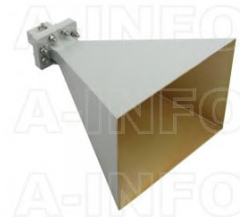
LB-OH-159-20-C-3.5F Octave Horn Antenna 4-8GHz 20dB Gain 3.5mm Female
