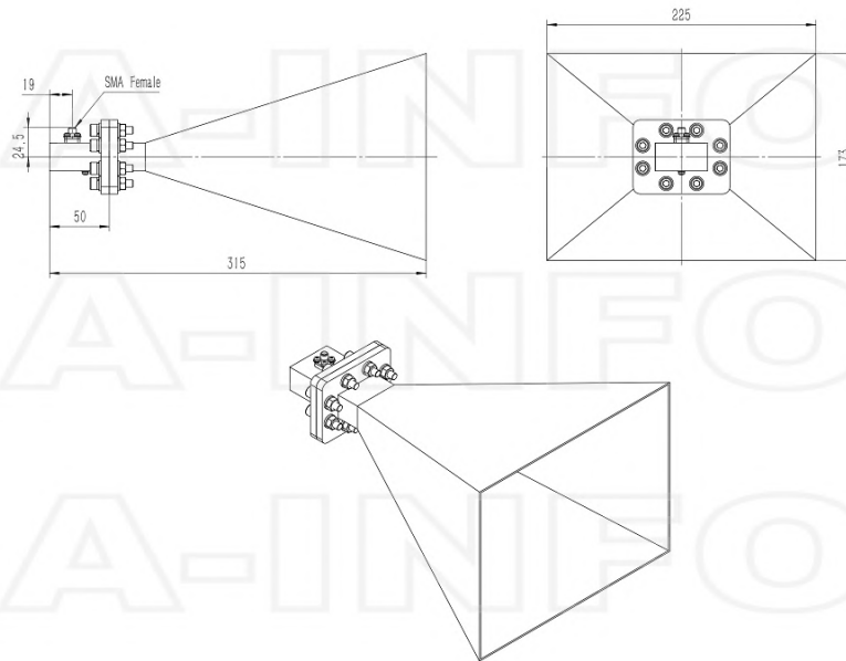
SMA-Female Output (P/N: LB-OH-159-20-C-SF)
