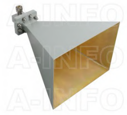
LB-OH-159-20-C-7 Octave Horn Antenna 4-8GHz 20dB Gain 7mm
