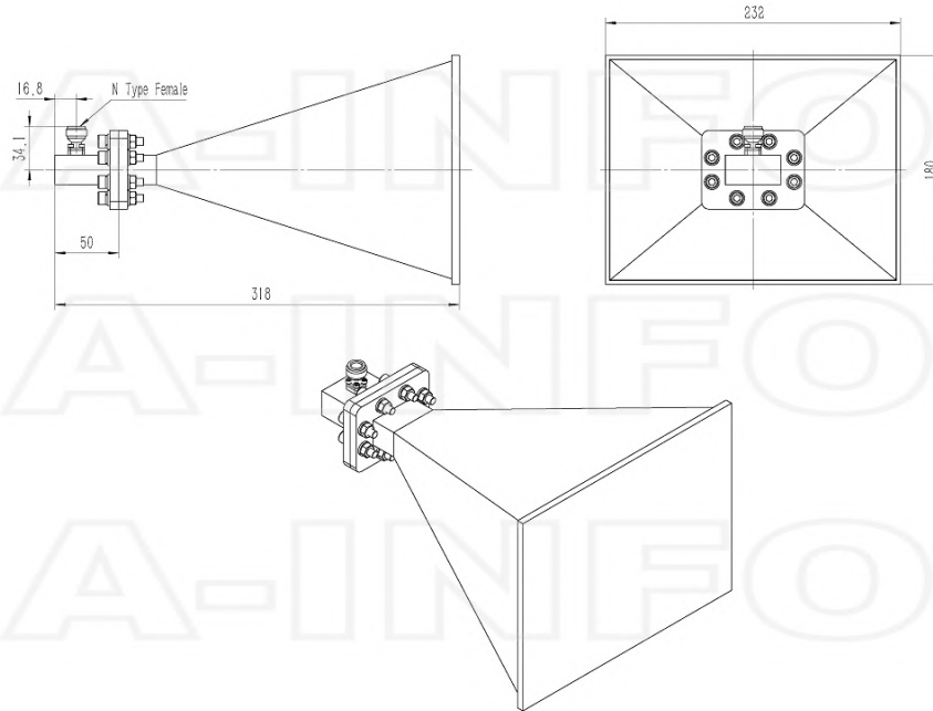
N-Female Output with Radome (Option, P/N: LB-OH-159-20-C-NFSPO, Outdoor Application)
