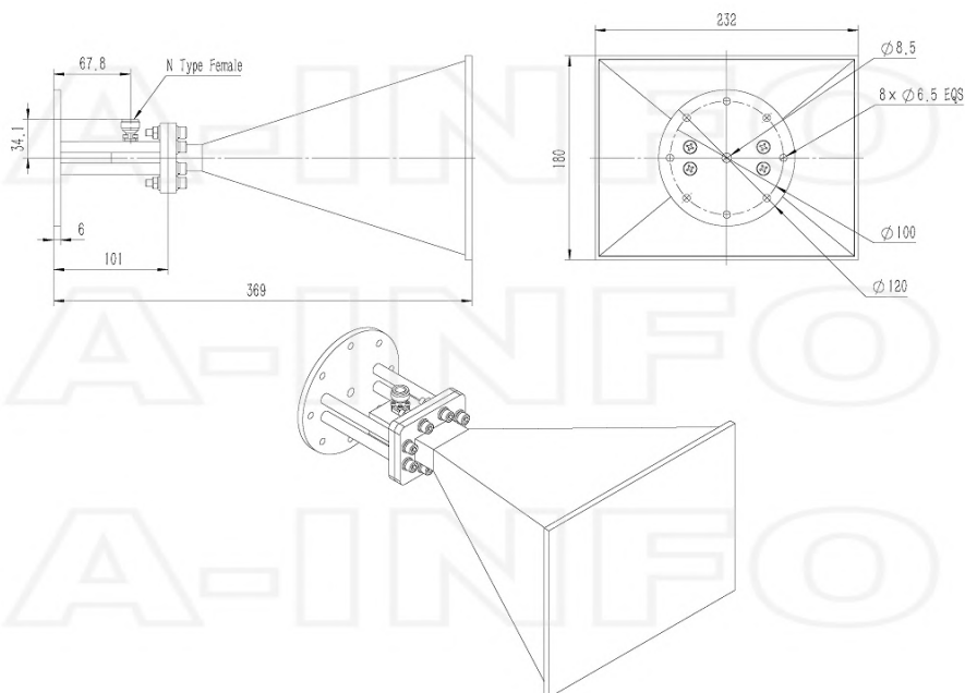
N-Female Output with Round Mounting Bracket & Radome (Option, P/N: LB-159-10-C-MB & LB-OH-159-20-C-NFSPO, Outdoor Application)
