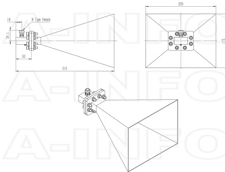
N-Female Output (P/N: LB-OH-159-20-C-NF)
