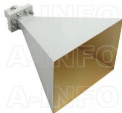
LB-OH-159-20-C-SF Octave Horn Antenna 4-8GHz 20dB Gain SMA Female
