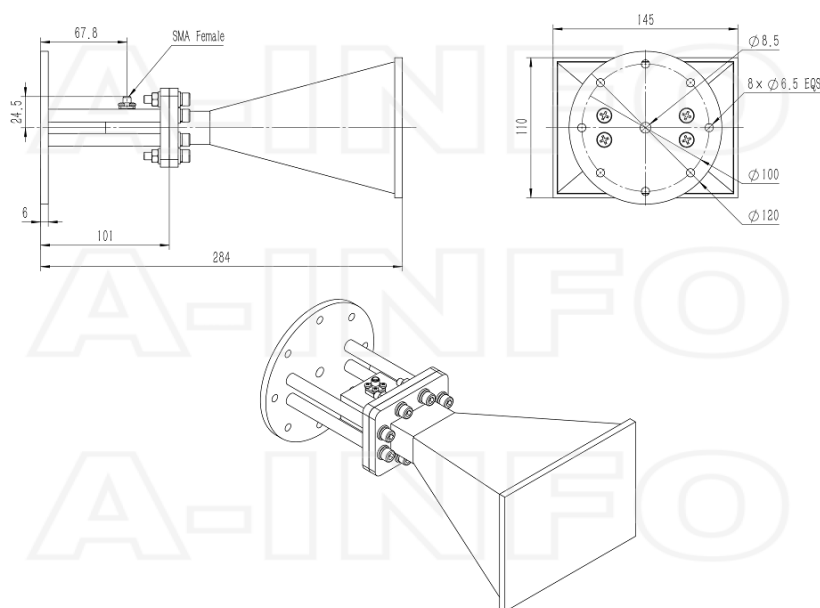
SMA-Female Output with Round Mounting Bracket & Radome (Option, P/N: LB-159-10-C-MB & LB-OH-159-15-C-SFSP0, Outdoor Application)
