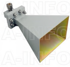
LB-OH-159-15-C-7 Octave Horn Antenna 4-8GHz 15dB Gain 7mm
