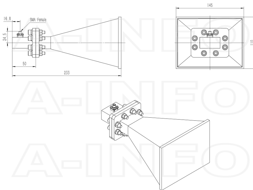
SMA-Female Output with Radome (Option, P/N: LB-OH-159-15-C-SFSP0, Outdoor Application)
