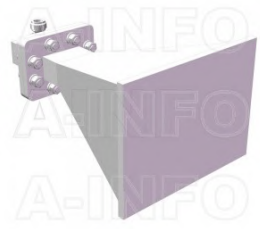
LB-OH-159-15-C-NFSPO Octave Horn Antenna 4-8GHz 15dB Gain N Type Female
