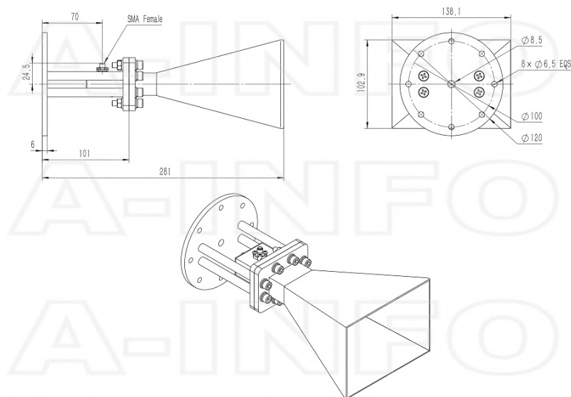
SMA-Female Output with Round Mounting Bracket (Option, P/N: LB-159-10-C-MB)
