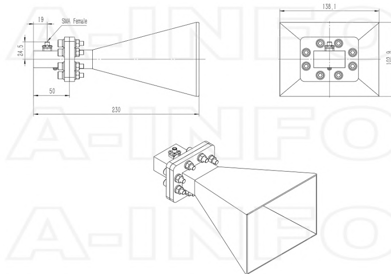
SMA-Female Output (P/N: LB-OH-159-15-C-SF)
