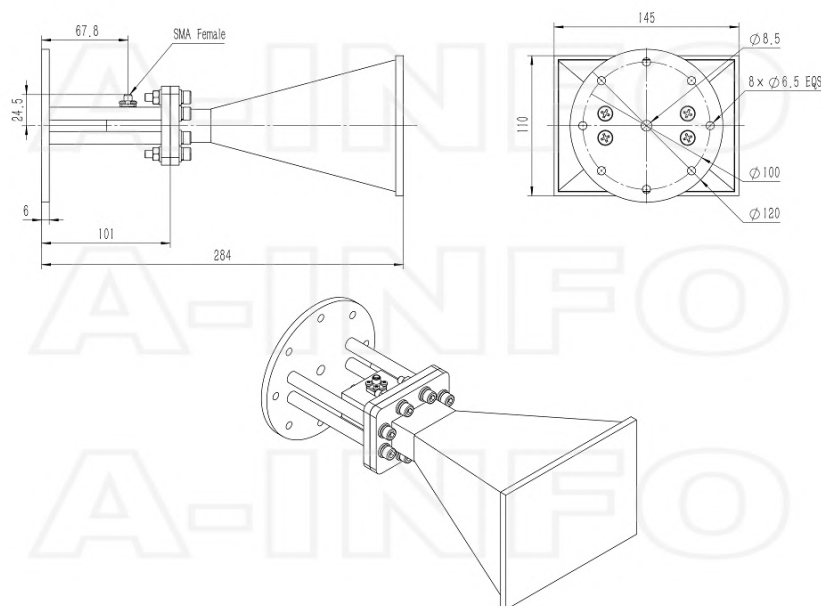
N-Female Output with Round Mounting Bracket & Radome (Option, P/N: LB-159-10-C-MB & LB-OH-159-15-C-NFSP0, Outdoor Application)
