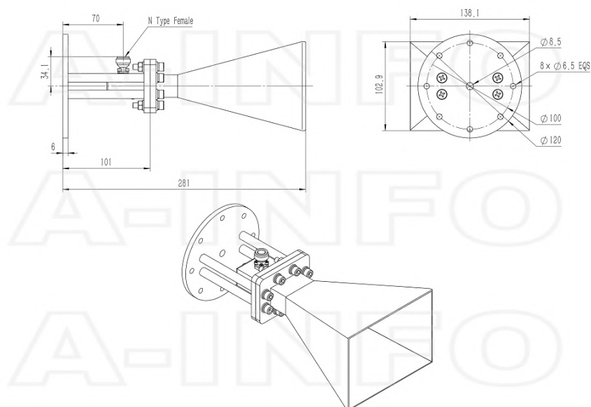
N-Female Output with Round Mounting Bracket (Option, P/N: LB-159-10-C-MB)
