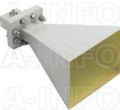
LB-OH-159-15-C-3.5F Octave Horn Antenna 4-8GHz 15dB Gain 3.5mm Female
