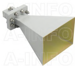
LB-OH-159-15-C-SF Octave Horn Antenna 4-8GHz 15dB Gain SMA Female
