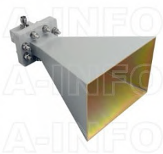
LB-OH-159-15-C-TF Octave Horn Antenna 4-8GHz 15dB Gain TNC Female
