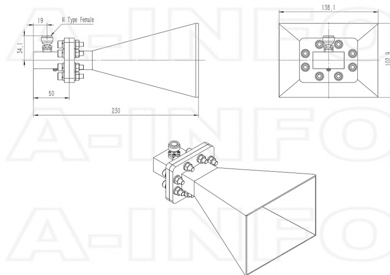
N-Female Output (P/N: LB-OH-159-15-C-NF)
