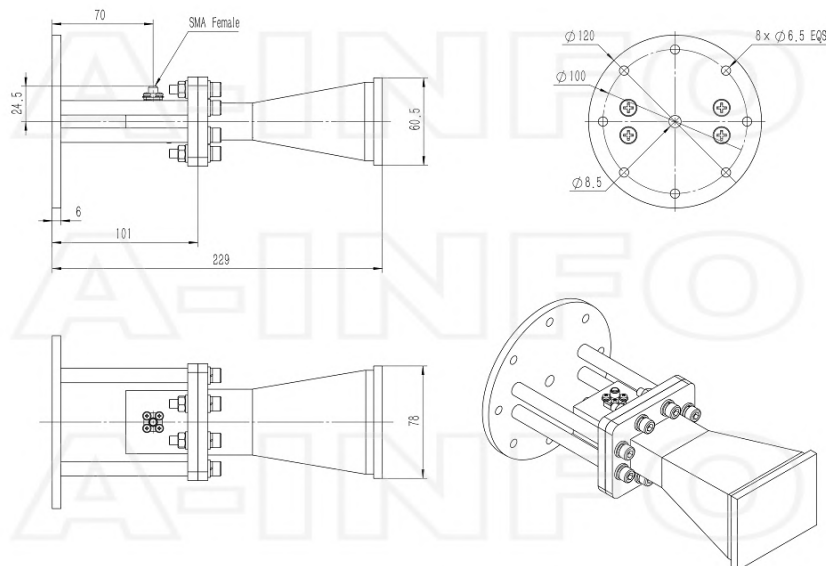
SMA-Female Output with Round Mounting Bracket & Radome (Option, P/N: LB-159-10-C-MB & LB-OH-159-10-C-SFSP0, Outdoor Application)
