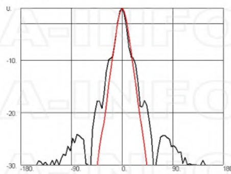
Frequency: 8.0 GHz
