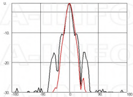
Frequency: 7.5 GHz
