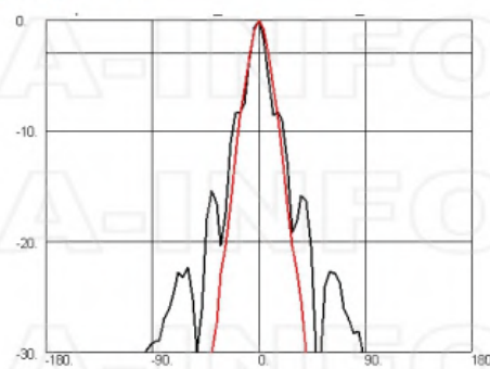
Frequency: 9.0 GHz
