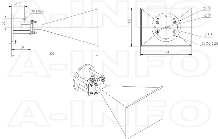
TNC-Female Output with Round Mounting Bracket & Radome (Option, P/N: LB-112-10-C-MB & LB-OH-112-20-C-TFSP0, Outdoor Application)
