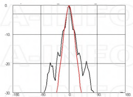
Frequency: 9.5 GHz
