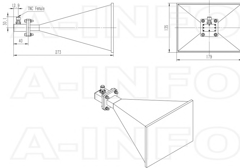
TNC-Female Output with Radome (Option, P/N: LB-OH-112-20-C-TFSP0, Outdoor Application)
