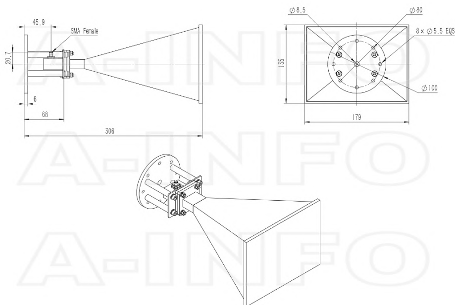
SMA-Female Output with Round Mounting Bracket & Radome (Option, P/N: LB-112-10-C-MB & LB-OH-112-20-C-SFSP0, Outdoor Application)
