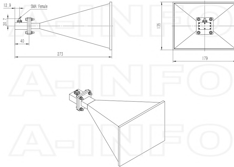
SMA-Female Output with Radome (Option, P/N: LB-OH-112-20-C-SFSP0, Outdoor Application)
