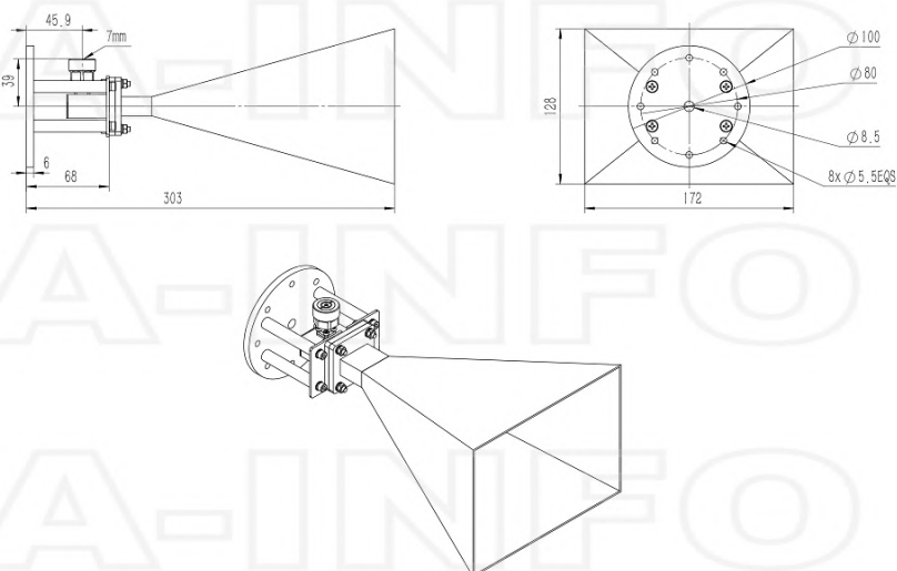
7mm Output with Round Mounting Bracket (Option, P/N: LB-112-10-C-MB)
