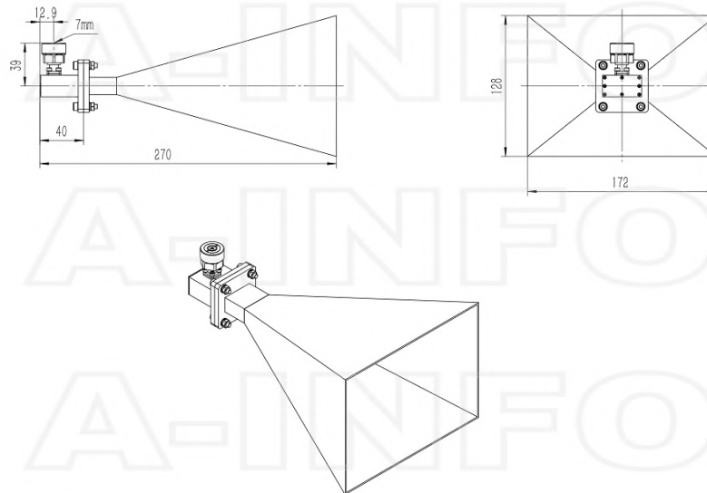
7mm Output (P/N: LB-OH-112-20-C-7)
