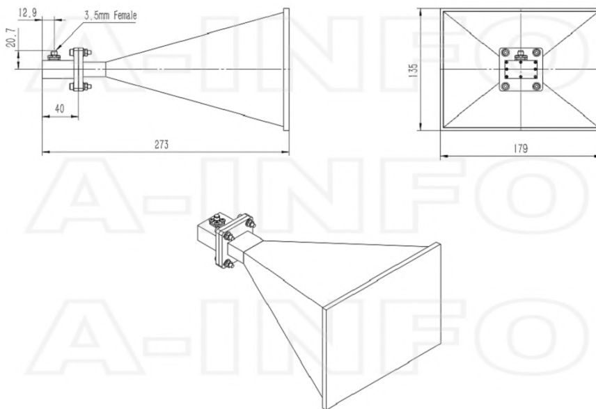
3.5mm-Female Output with Radome (Option, P/N: LB-OH-112-20-C-3.5FSPO, Outdoor Application)
