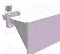
LB-OH-112-15-C-7SPO Octave Horn Antenna 6-12GHz 15dB Gain 7mm
