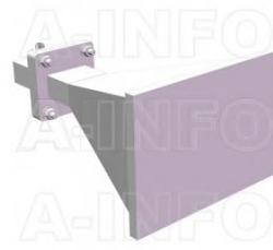
LB-OH-112-15-C-SFSP0 Octave Horn Antenna 6-12GHz 15dB Gain SMA Female
