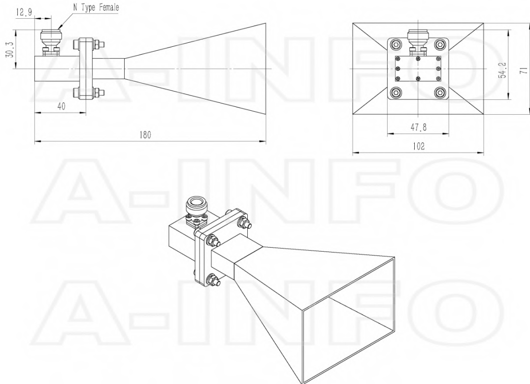
N-Female Output (P/N: LB-OH-112-15-C-NF)
