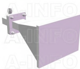
LB-OH-112-15-C-TFSP0 Octave Horn Antenna 6-12GHz 15dB Gain TNC Female
