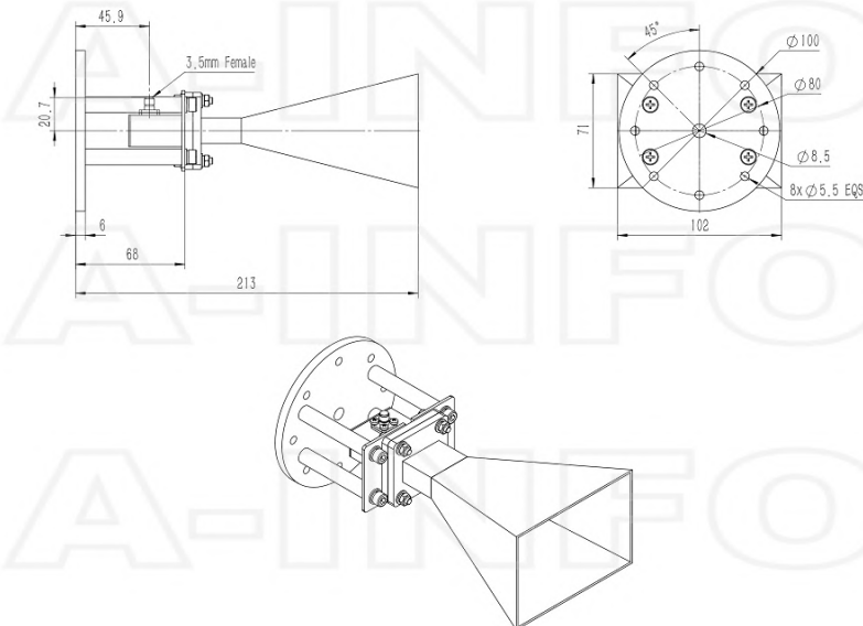
3.5mm-Female Output with Round Mounting Bracket (Option, P/N: LB-112-10-C-MB)
