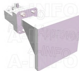
LB-75180-10-C-SFSP Multi Octave Horn Antenna 7.5-18GHz 10dB Gain SMA Female
