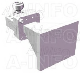
LB-75180-10-C-NFSPO Multi Octave Horn Antenna 7.5-18GHz 10dB Gain N Type Female
