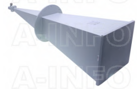
LB-65180-25-C-NFSPO Multi Octave Horn Antenna 6.5-18GHz 25dB Gain N Type Female
