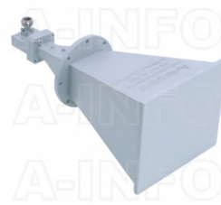
LB-65180-20-C-NFSPO Multi Octave Horn Antenna 6.5-18GHz 20dB Gain N Type Female
