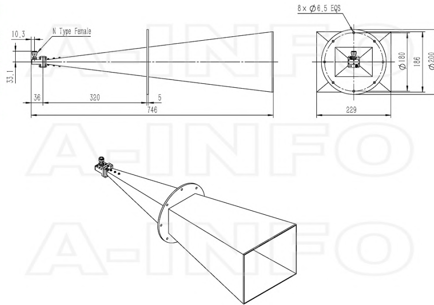
N-Female Output (P/N: LB-60180-25-C-NF)
