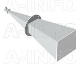
LB-60180-25-C-HNFSPO Multi Octave Horn Antenna 6.0-18.0GHz 25dB Gain High Power N Type Female
