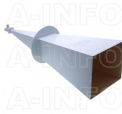
LB-60180-25-C-HNF Multi Octave Horn Antenna 6.0-18.0GHz 25dB Gain High Power N Type Female
