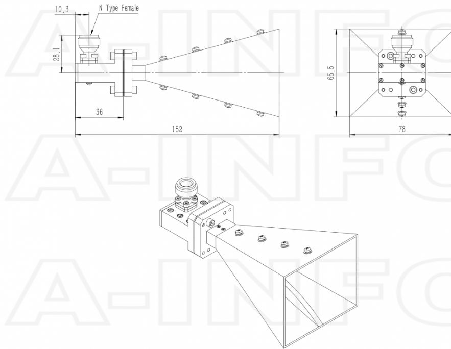
N-Female Output (P/N: LB-60180-15-C-NF)
