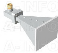
LB-60180-15-C-HNFSPO Multi Octave Horn Antenna 6.0-18.0GHz 15dB Gain High Power N Type Female
