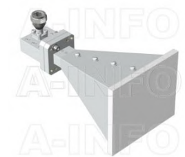
LB-60180-15-C-NFSPO Multi Octave Horn Antenna 6.0-18.0GHz 15dB Gain N Type Female
