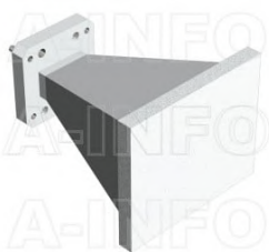
LB-60180-10-ASPO Multi Octave Horn Antenna 6.0-18.0GHz 10dB Gain Double Ridge Waveguide Interface
