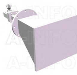
LB-58160-20-C-NFSPO Multi Octave Horn Antenna 5.8-16GHz 20dB Gain N Type Female
