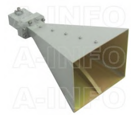
LB-475110-15-C-SF Multi Octave Horn Antenna 4.75-11GHz 15dB Gain SMA Female
