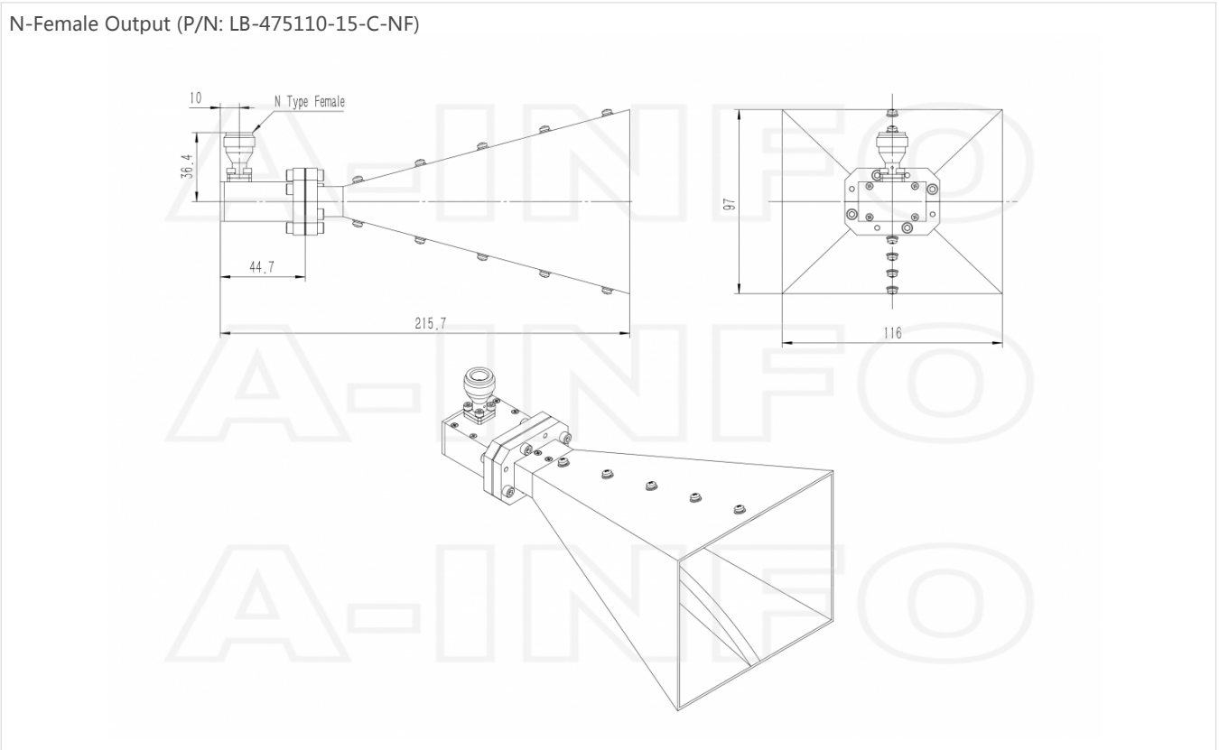
N-Female Output with Round Mounting Bracket (Option, P/N: LB-475110-10-C-MB)
