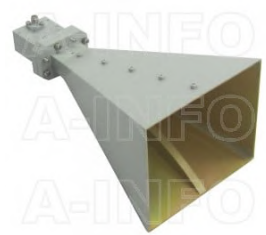
LB-475110-15-C-SF Multi Octave Horn Antenna 4.75-11GHz 15dB Gain SMA Female
