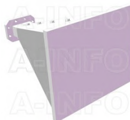
LB-475110-15-ASPO Multi Octave Horn Antenna 4.75-11GHz 15dB Gain Double Ridge Waveguide Interface
