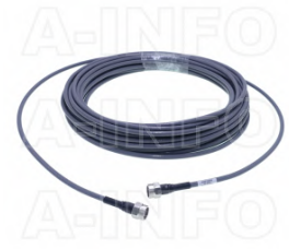
NM-NM-A100-20000 Flexible Cable Assembly 20000mm DC-18GHz N Male to N Male
