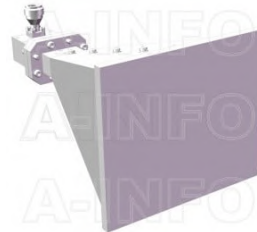
LB-475110-15-C-NFSPO Multi Octave Horn Antenna 4.75-11GHz 15dB Gain N Type Female
