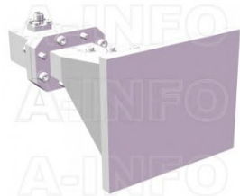
LB-475110-10-C-SFSP0 Multi Octave Horn Antenna 4.75-11GHz 10dB Gain SMA Female
