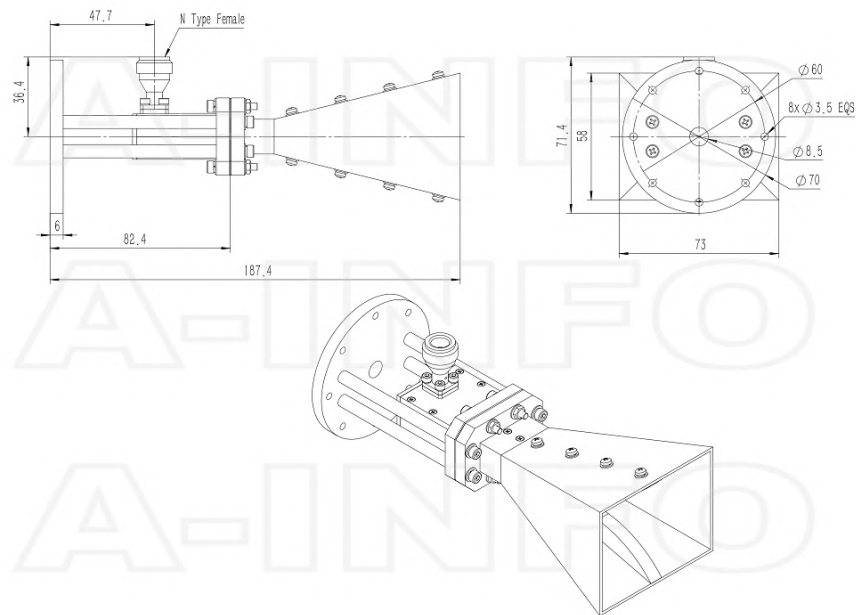
N-Female Output with Round Mounting Bracket (Option, P/N: LB-475110-10-C-MB)
