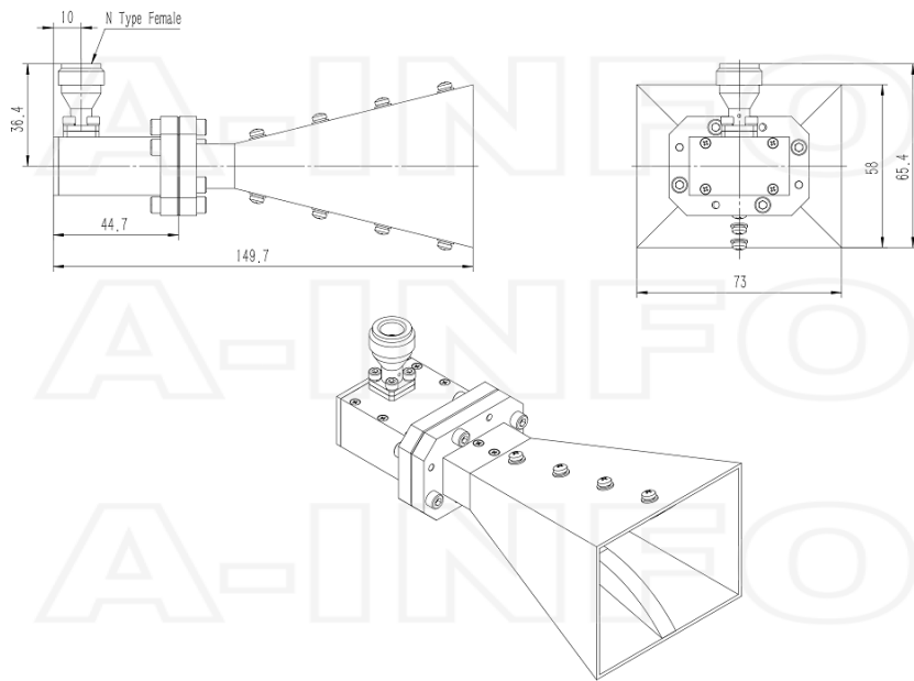
N-Female Output (P/N: LB-475110-10-C-NF)
