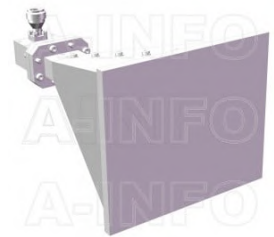
LB-3582-15-C-NFSP0 Multi Octave Horn Antenna 3.5-8.2GHz 15dB Gain N Type Female
