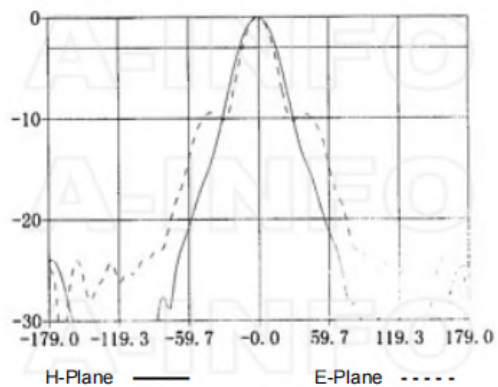
Frequency: 4.5GHz
