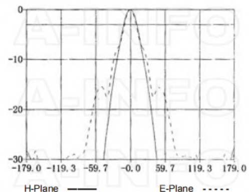
Frequency: 7.0GHz
