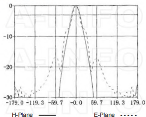
Frequency: 6.5GHz
