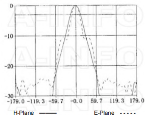
Frequency: 5.0GHz
