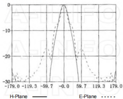
Frequency: 6.5GHz
