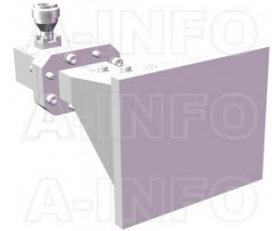
LB-3582-10-C-NFSP0 Multi Octave Horn Antenna 3.5-8.2GHz 10dB Gain N Type Female
