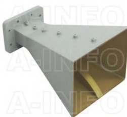
LB-3582-10-A Multi Octave Horn Antenna 3.5-8.2GHz 10dB Gain Double Ridge Waveguide Interface
