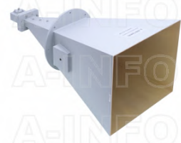
LB-2678-20-C-SF Multi Octave Horn Antenna 2.6-7.8GHz 20dB Gain SMA Female
