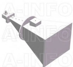
LB-2678-20-C-SFSP0 Multi Octave Horn Antenna 2.6-7.8GHz 20dB Gain SMA Female
