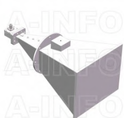
LB-2678-20-C-SFSPO Multi Octave Horn Antenna 2.6-7.8GHz 20dB Gain SMA Female
