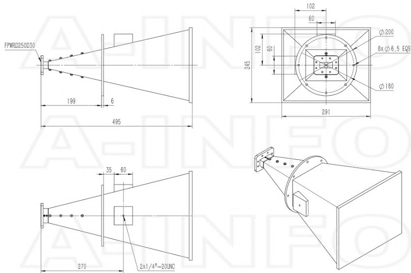
FPWRD250D30 Output with Radome (Option, P/N: LB-2678-20-ASPO, Outdoor Application)
