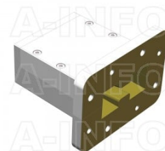
250DRWECAS Endlaunch Double Ridge Waveguide to Coaxial Adapter 2.6-7.8GHz WRD250 to SMA Female
