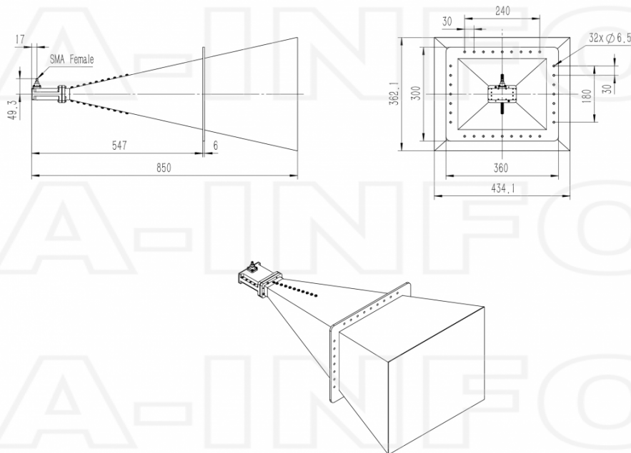
SMA-Female Output (P/N: LB-2048-20-C-SF)
