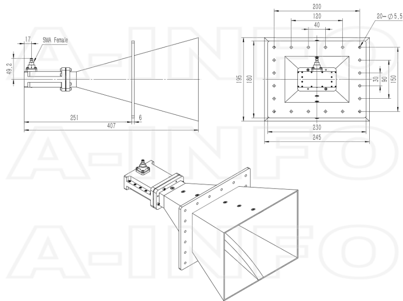
SMA-Female Output (P/N: LB-2048-15-C-SF)
