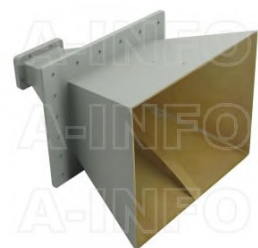
LB-2048-15-A Multi Octave Horn Antenna 2-4.8GHz 15dB Gain Double Ridge Waveguide Interface
