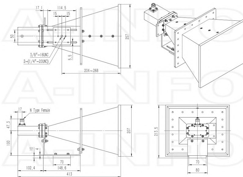
N-Female Output with L Type Mounting Bracket & Radome (Option, P/N: LB-2048-15-C-L & LB-2048-15-C-NFSPO, Outdoor Application)
