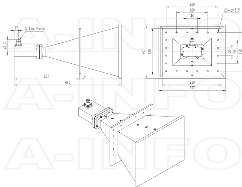
N-Female Output with Radome (Option, P/N: LB-2048-15-C-NFSPO, Outdoor Application)
