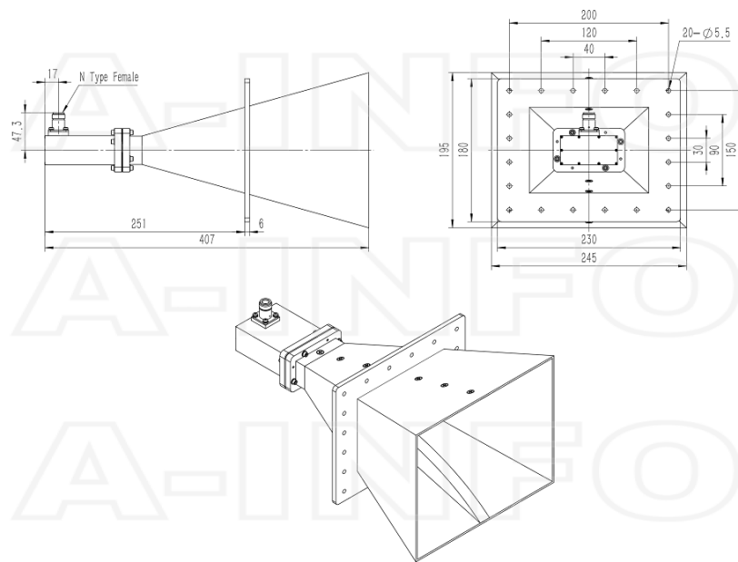
N-Female Output (P/N: LB-2048-15-C-NF)
