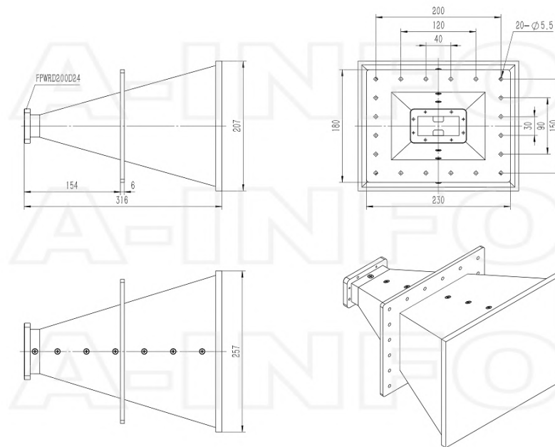
FPWRD200D24 Output with Radome (Option, P/N: LB-2048-15-ASPO, Outdoor Application)
