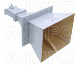
LB-2048-15-C-SF Multi Octave Horn Antenna 2-4.8GHz 15dB Gain SMA Female
