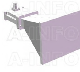
LB-2048-10-C-NFSPO Multi Octave Horn Antenna 2-4.8GHz 10dB Gain N Type Female
