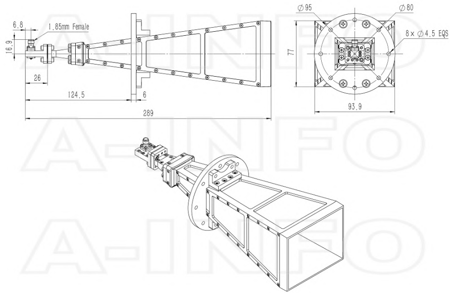
1.85mm-Female Output (P/N: LB-180550-25-C-1.85F)
