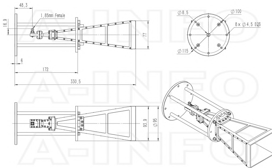
1.85mm-Female Output with Round Mounting Bracket (Option, P/N: LB-180400-25-MB2)
