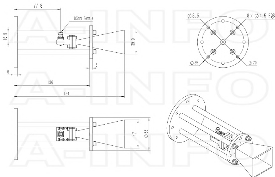
1.85mm-Female Output with Round Mounting Bracket (Option, P/N: LB-19-25-MB2)
