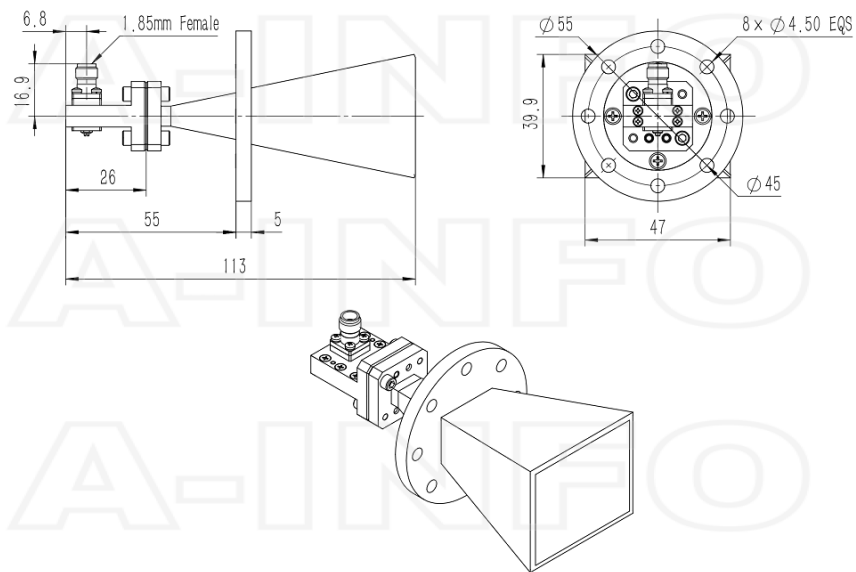
1.85mm-Female Output (P/N: LB-180550-20-C-1.85F)
